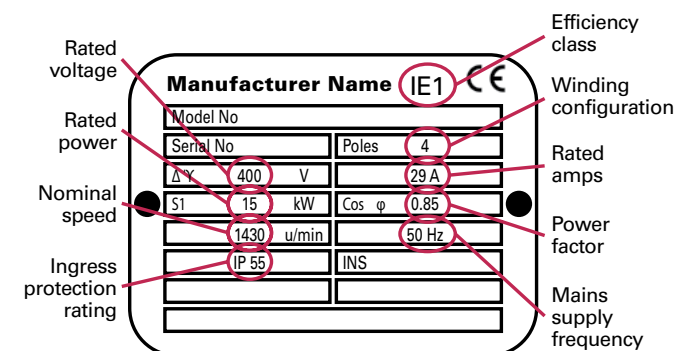
Figure 2 Typical information provided on a motor name plate
