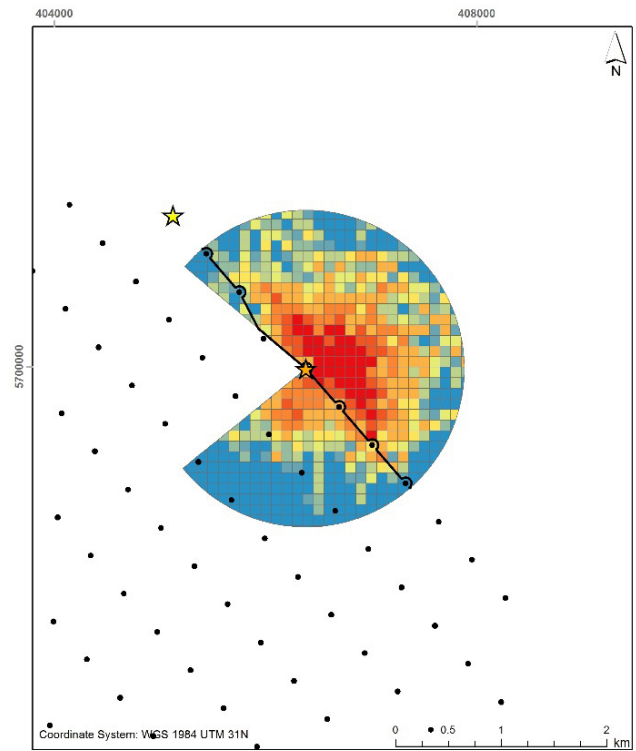
G05 RF Black-legged Kittiwake - Track length/km 2
