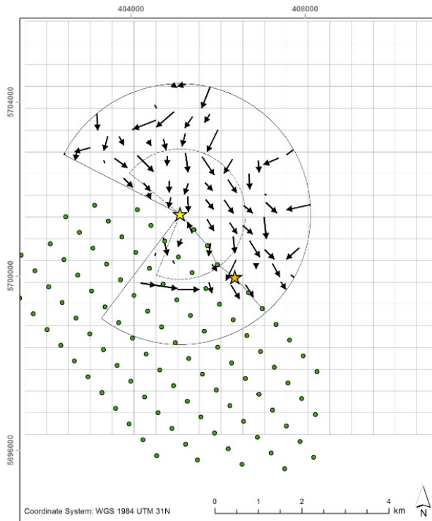
Figure 6.9. Flight directions for Black-legged Kittiwake recorded from turbine G01.
