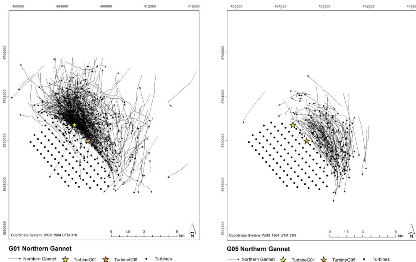
Figure 6.1. Northern Gannets flight tracks collected using the SCANTER radar and LAWR radar from turbines G01 (left) and G05 (right) respectively.
