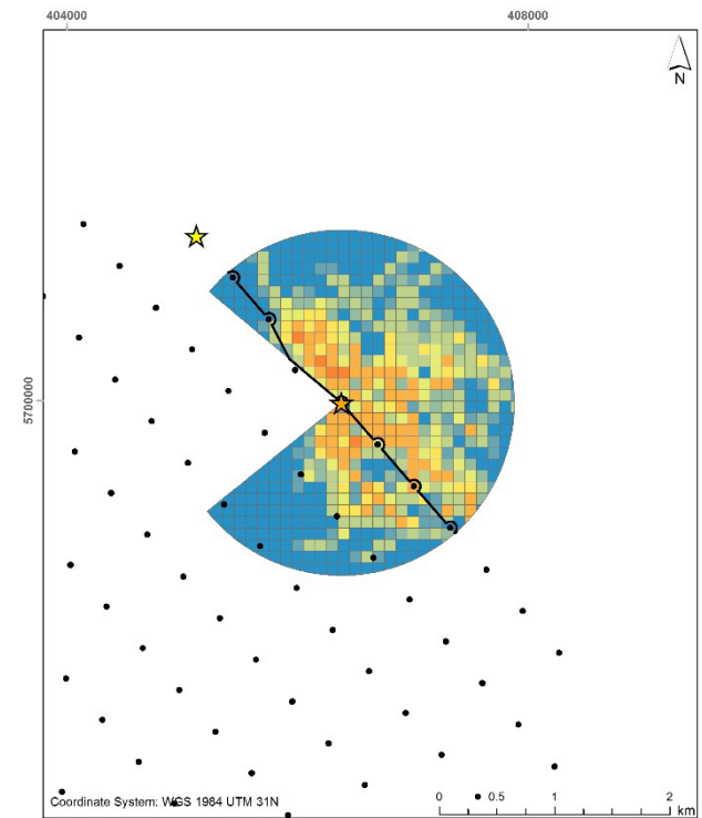
G05 RF Lesser Black-backed Gull - Track length/km 2
