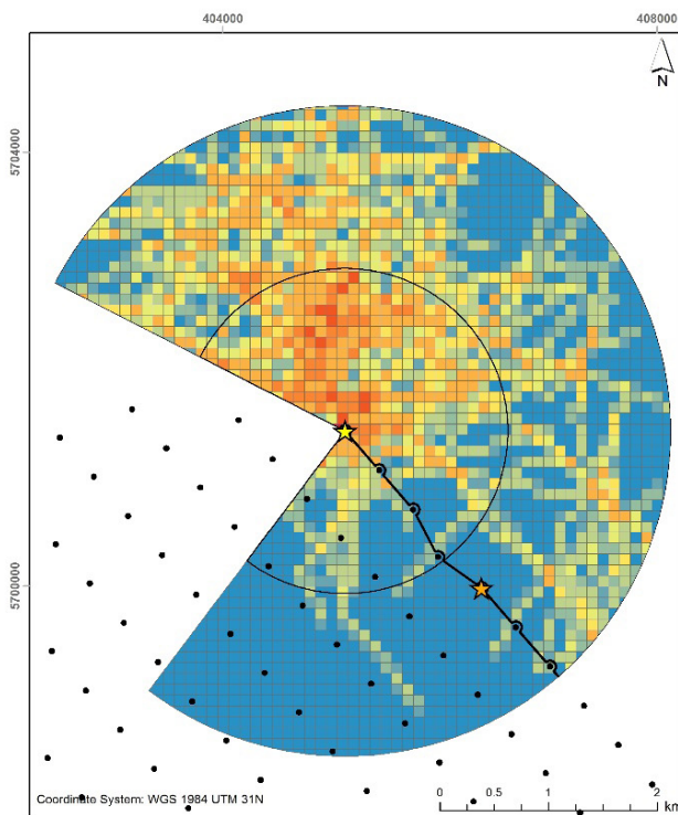
Figure 6.12. Lesser Black-backed gull track density (calculated through track length per unit area method) based on data collected using the SCANTER radar and LAWR radar from turbines G01 (left) and G05 (right) respectively.
