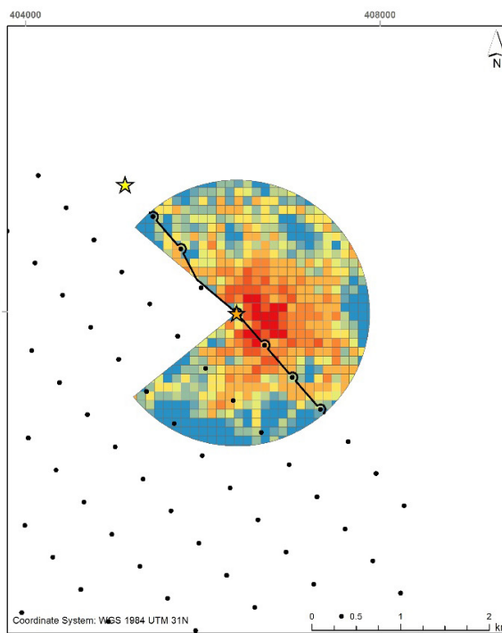
G05 RF Herring Gull - Track length/km 2
