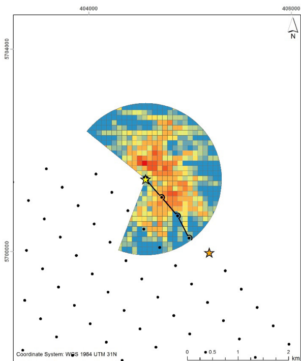
G01 RF Herring Gull - Track length/km 2
