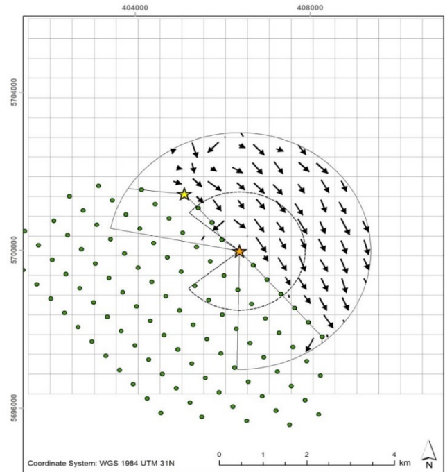
Mean direction of Gannet flight tracks in 500 m grid cells ★ TurbineG01 → G05 radar Gannet mean dir. □ G05 1.5km buffer ★ TurbineG05 □ 500 m grid □ G05 3km buffer ● Turbines
