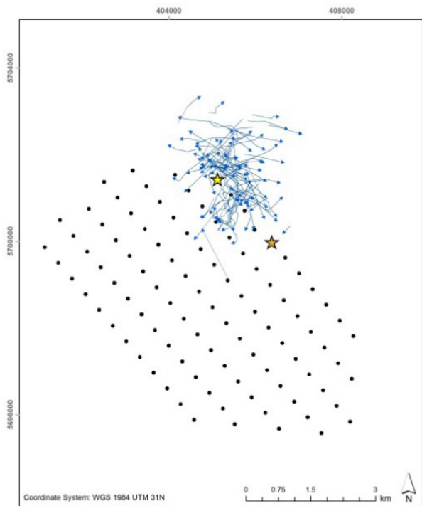
G01 Herring Gull rangefinder tracks
