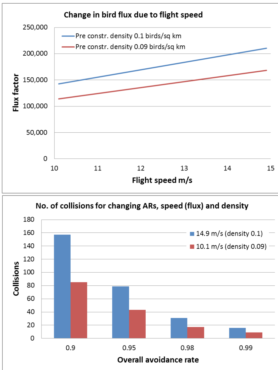
Figure 2. The below graph illustrates changes in flux factor against a range of flight speeds, for two pre-construction densities. The lower graph illustrates the difference between a “high collision risk” scenario (14.9 m/s and 0.1 birds/km 2 ) and a “low collision risk scenario” (10.1 m/s and 0.09 birds/km 2 ), from the upper graph, against four different avoidance rates.
